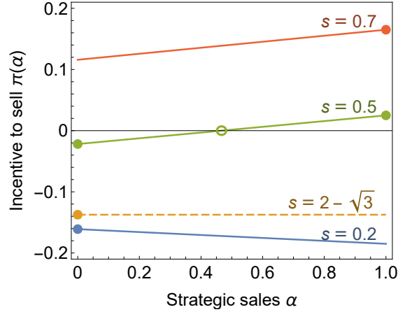
Figure 2: Incentive to sell and equilibria. The figure shows the payoff gain \pi(\alpha) for different values of liquidity risk s . Circles indicate equilibria of the game under complete information. Parameters: c = 0.25 , v = 1.2 .
