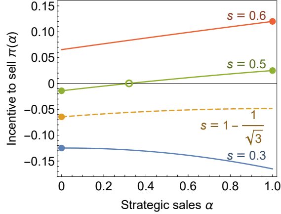
Figure 10: Pooled trade execution and cubic balance sheet costs. The figure shows the payoff gain \pi(\alpha) for different values of liquidity risk s . Circles indicate equilibria of the game under complete information. Parameters: v = 1.2 , c = 0.25 .
