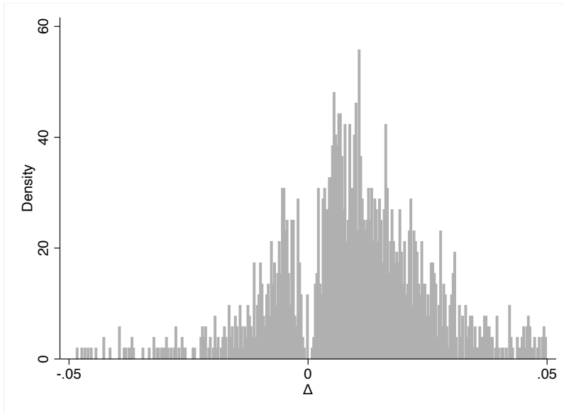
Figure 1: Distribution of bid differences \Delta
