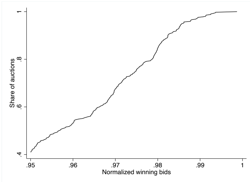
Figure 2: Cumulative distribution function of normalized winning bids
