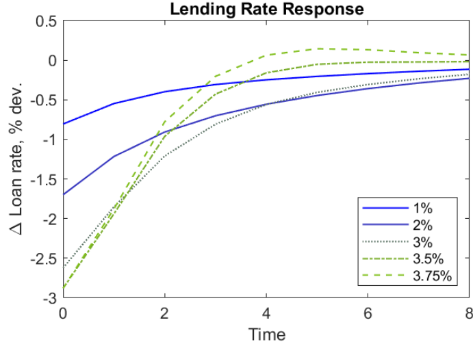
Figure 3: Impulse response of loan rates to Taylor rule innovations of increasing size, in deviations from the steady state. The legend contains the size of the respective innovations to the Taylor rule. The dashed line reflects a reversal of the response, including on impact. For the largest shock, the policy rate reaches about -1\% on impact. The dotted line shows that a reversal occurs even for smaller innovations but at a later horizon, in line with our “creeping up” result.
