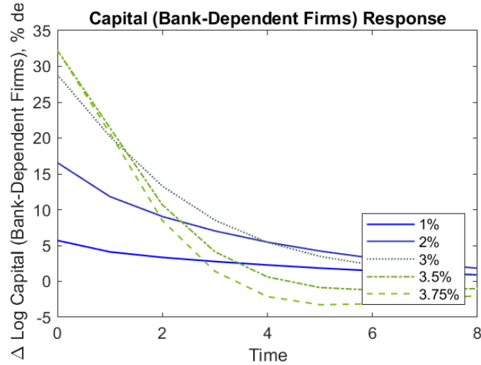
Figure 4: Impulse response of log capital of new bank-dependent firms to Taylor rule innovations of increasing size, in deviations from the steady state. The legend contains the size of the respective innovations to the Taylor rule. The dashed line reflects a reversal of the response, including on impact. For the largest shock, the policy rate reaches about -1\% on impact. The dotted line shows that a reversal occurs even for smaller innovations but at a later horizon, in line with our “creeping up” result.
