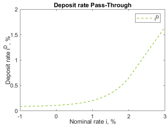
Figure 8: Pass-through of nominal rates into deposit rates given the calibrated values of \eta_1, \eta_2, \eta_3 . The pass-through is assumed to be one-for-one for policy rates above the steady state ( i > i^{SS} ).
